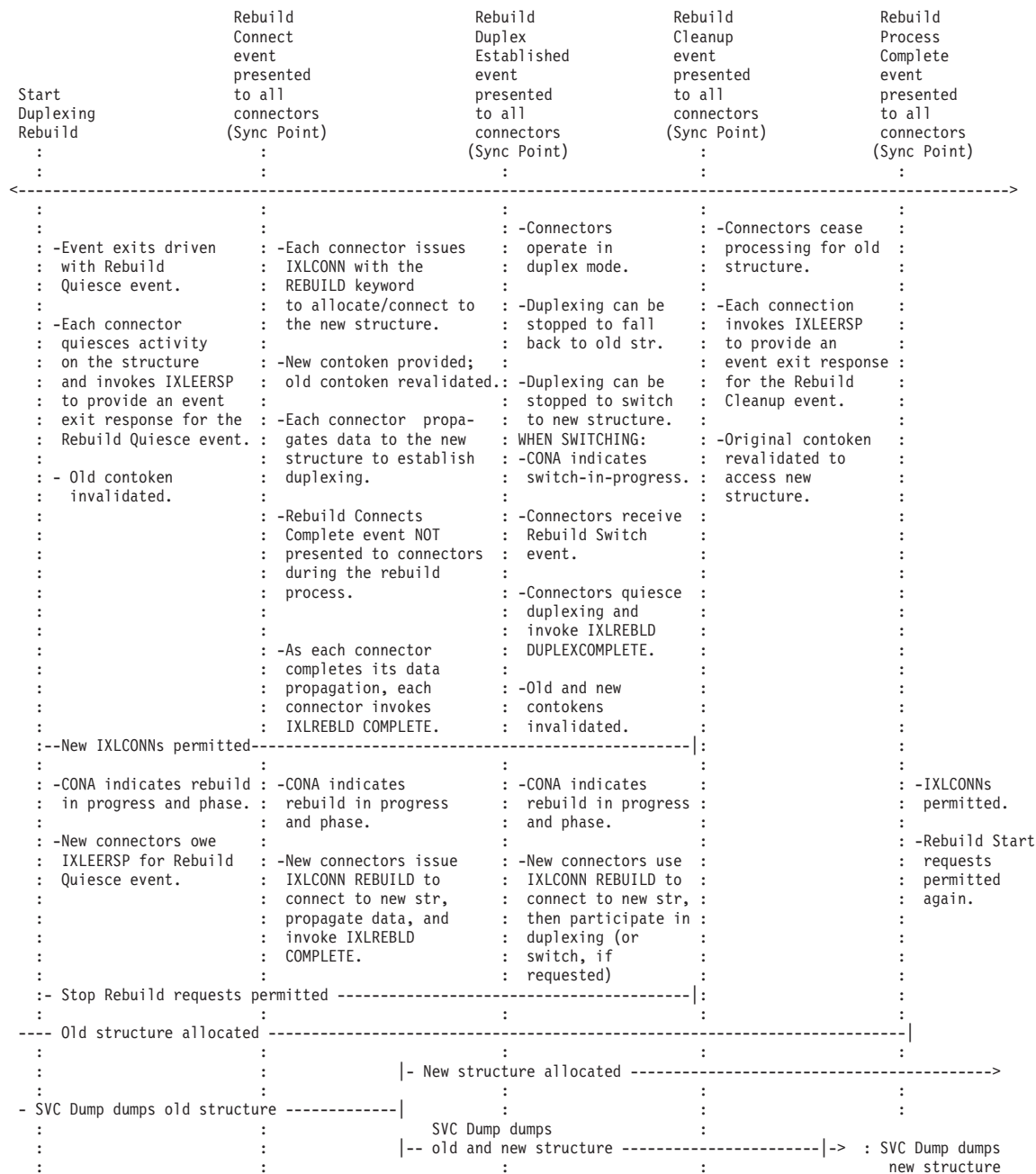
Figure 25. User-Managed Duplexing Rebuild Timeline
