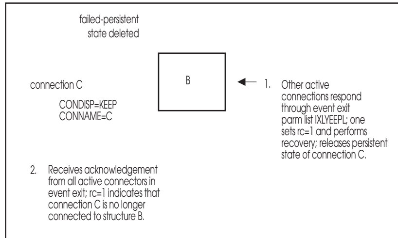
Figure 23. Deleting a Failed-Persistent Connection using IXL YEEPL
