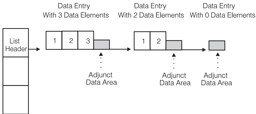
Figure 37. List Containing Entries with Various Numbers of Data Elements. List entry controls not shown.
