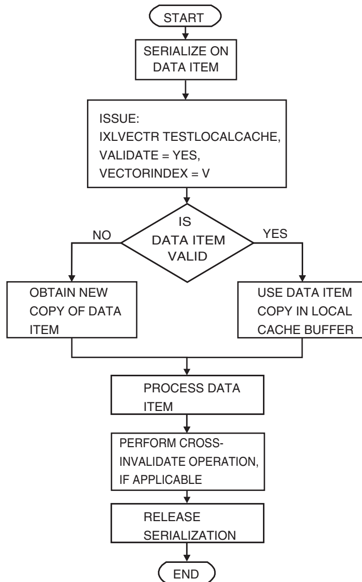
Figure 70. Sample Serialization Protocol for Single Data Item
