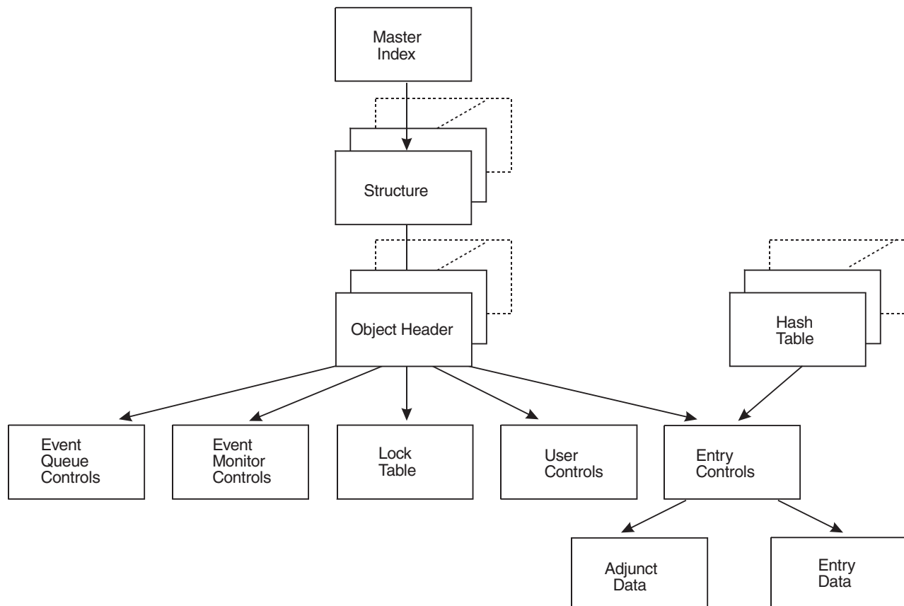
Figure 74. Format of Coupling Facility Structure Data in Dump Data Set
