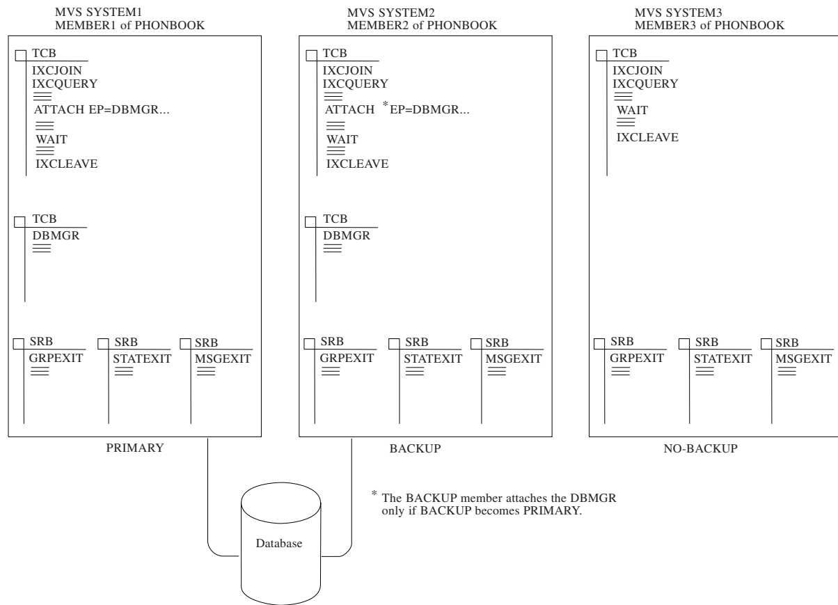
Figure 11. PHONBOOK Multisystem Application
