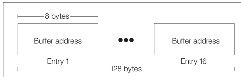
Figure 33. Format of Buffer List (BUFLIST) - 64-bit Addresses
