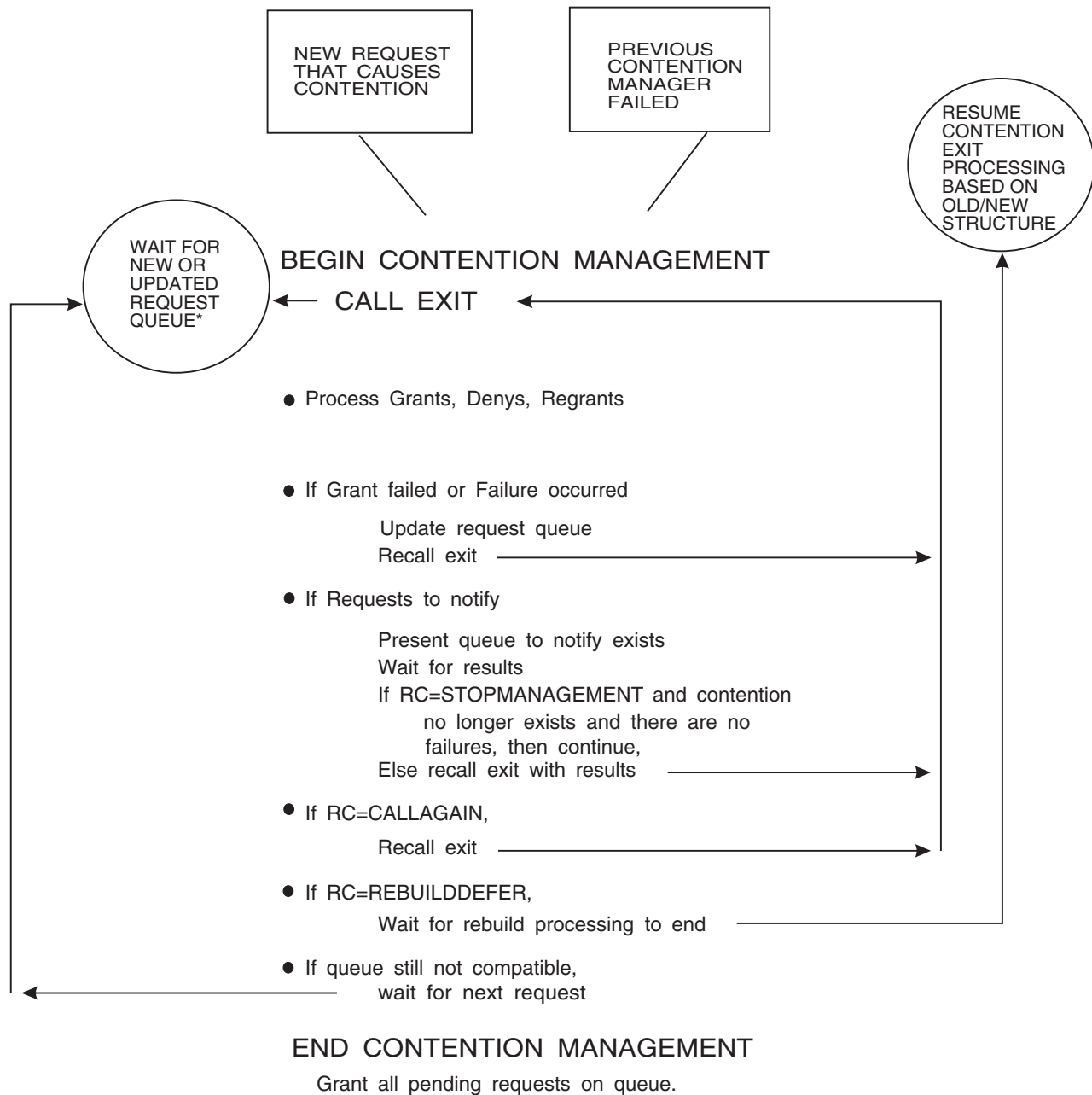
Figure 69. Contention Exit Processing
