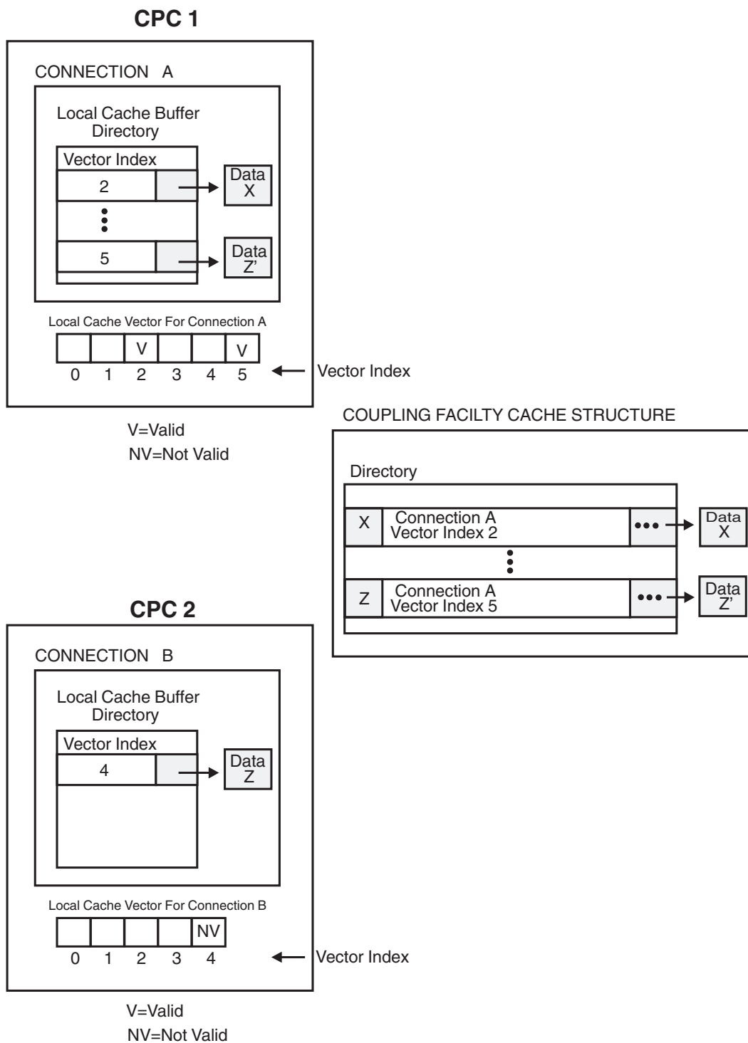
Figure 31. Invalidating Local Cache Copy of a Data Item
