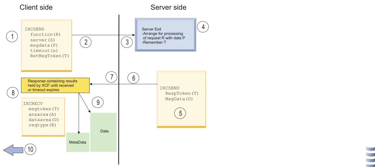
Figure 13. Overview of client/server processing in the sysplex
