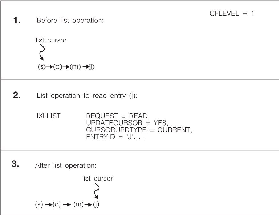
Figure 47. Updating the List Cursor to the Current Entry — Example 1
