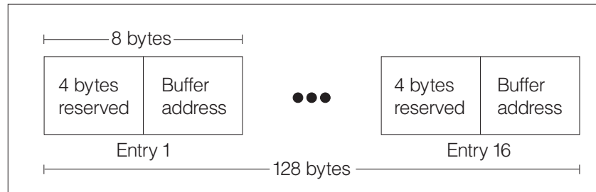
Figure 32. Format of Buffer List Specified by the BUFLIST Parameter
