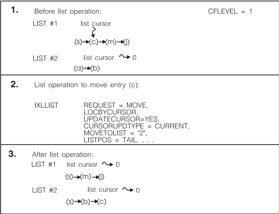
Figure 48. Updating the List Cursor to the Current Entry — Example 2
