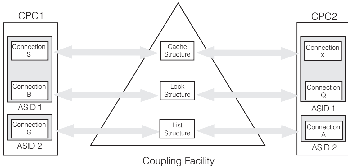
Figure 14. Multiple Systems Sharing Data Through a Coupling Facility
