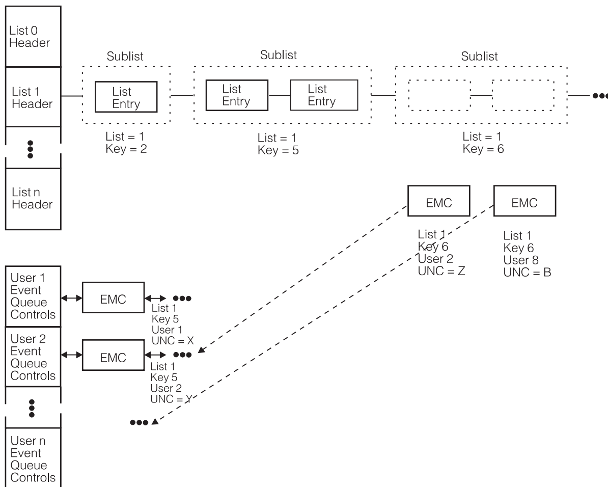
Figure 36. Event Queues in a List Structure
