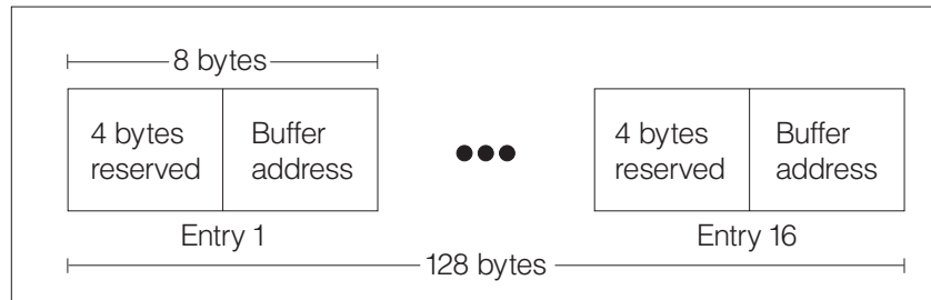
Figure 59. Format of Buffer List Specified by the BUFLIST Parameter
