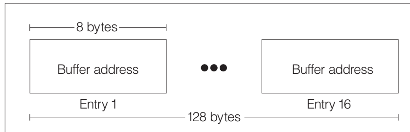
Figure 60. Format of Buffer List - 64-bit Addresses
