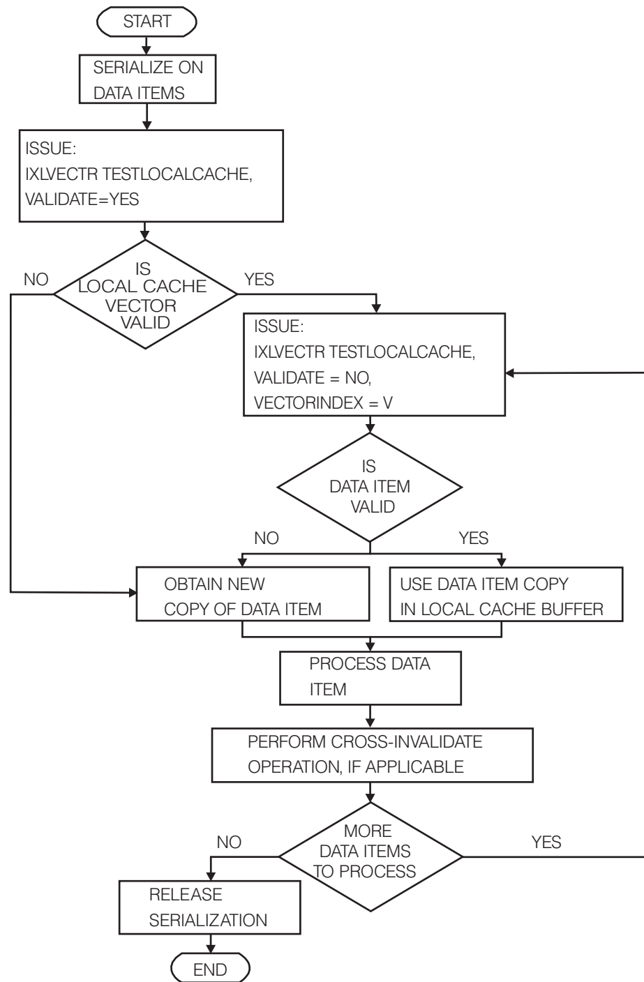
Figure 71. Sample Serialization Protocol for Multiple Data Items
