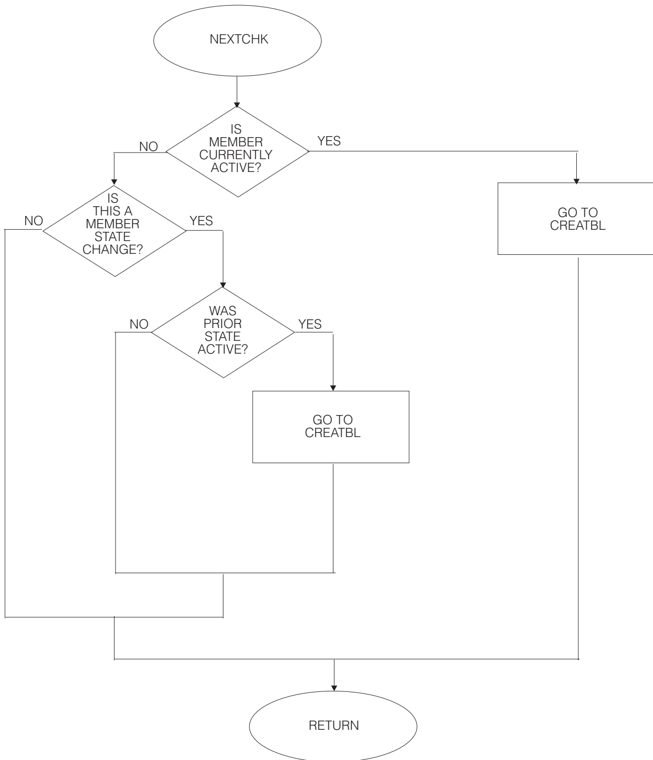
Figure 10. Summary of Group User Routine Logic (Part 2 of 3)
